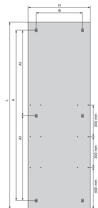
Heaters with 1.800 mm height
