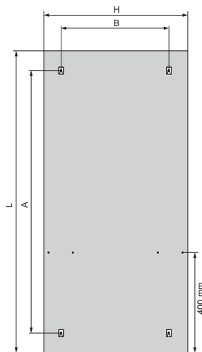
Heaters with 1.200 mm height
