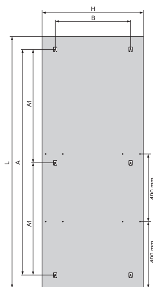
Heaters with 1.500 mm height
